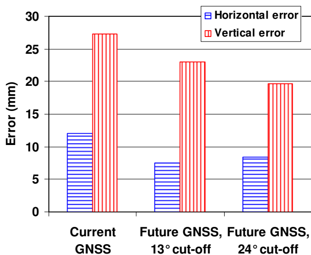
Figure 7: Horizontal and vertical positioning errors, with current and future GNSS constellations.
