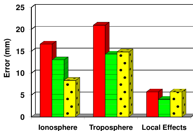
Figure 8 (Emardson et al., 2009b): Vertical error contribution from the three major error sources, for nominal (red), new GNSS (green striped) and network densified (yellow dotted) cases respectively.
