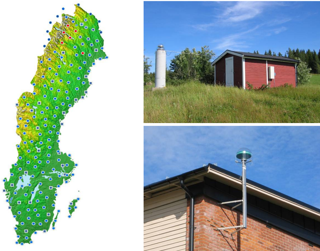
Figure 1: Left: Current SWEPOS network and a number of bordering Norwegian and Finnish stations that are used in SWEPOS Network-RTK Service. Blue squares are stations of Class A type. Blue dots are stations of Class B type, established step-by-step for network-RTK purposes. Red dots are Class B stations which are planned in the near future.
