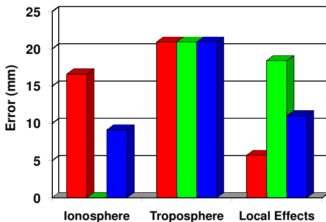
Figure 5 (Emardson et al., 2009b): Vertical error contribution from the three major error sources, for L1 (red), L3 (green) and L 0 (blue).
