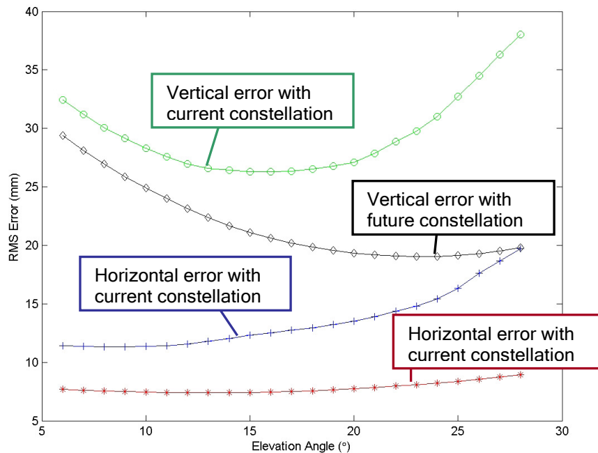
Figure 6 (adapted from Emardson et al., 2009a): RMS error as a function of elevation angle for the horizontal and vertical components.
