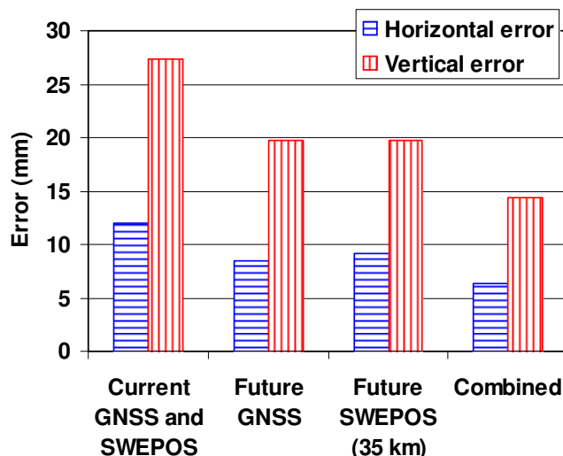
Figure 9: Horizontal and vertical positioning errors, with current and future GNSS constellations.
